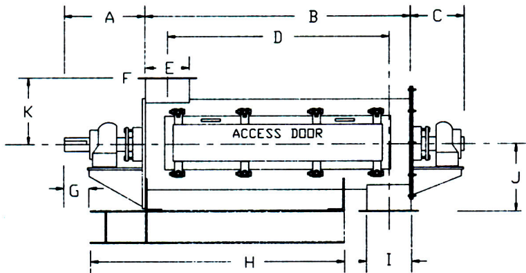
HIGH SPEED BLENDER DIMENSIONS (IN)
